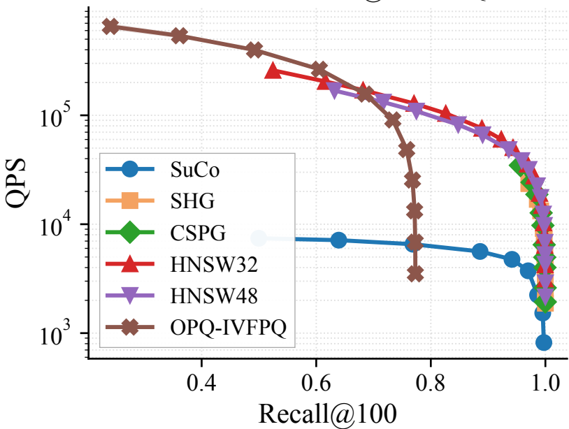
DEEP1M — Recall@100 vs QPS
