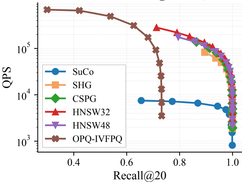
DEEP1M — Recall@20 vs QPS
