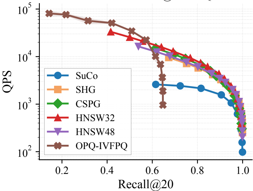
GIST1M — Recall@20 vs QPS
