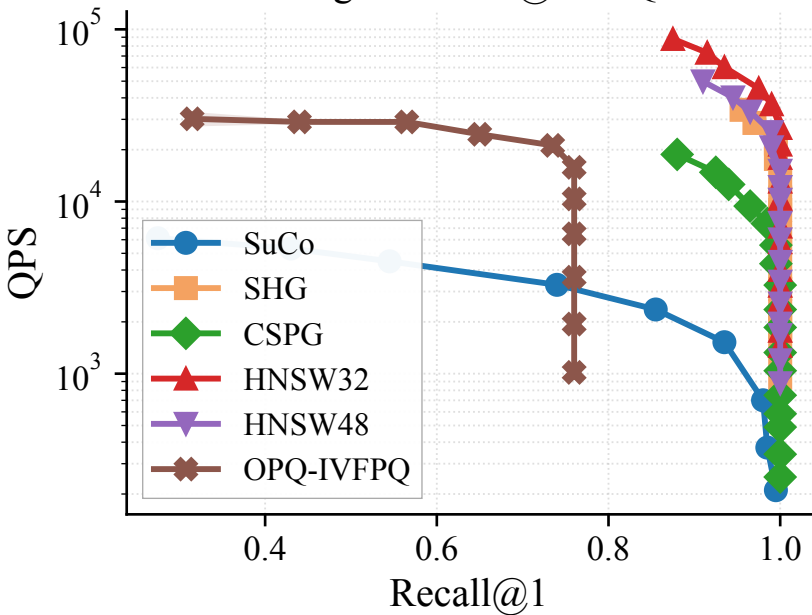
MSong — Recall@1 vs QPS
