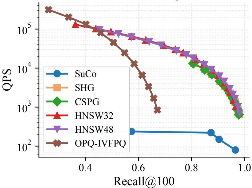
MSTuring10M — Recall@100 vs QPS
