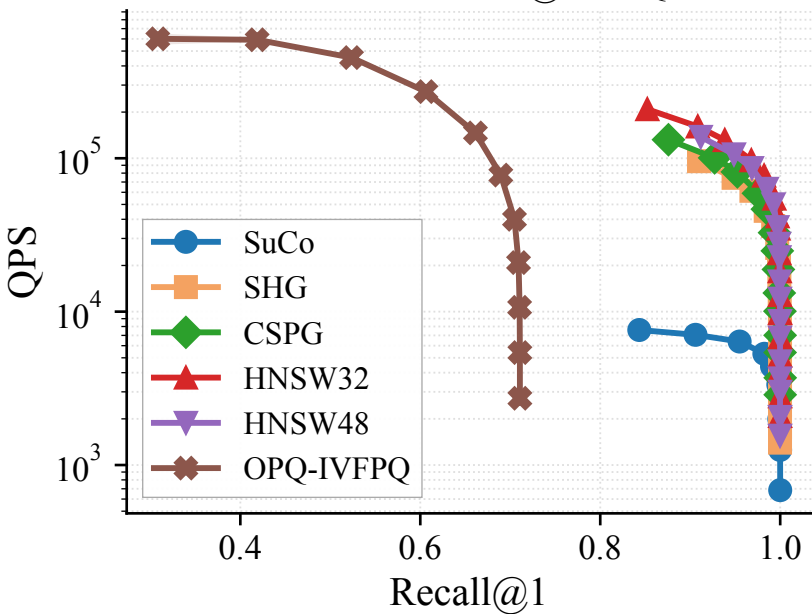
SIFT1M — Recall@1 vs QPS
