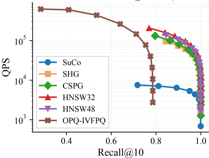
SIFT1M — Recall@10 vs QPS
