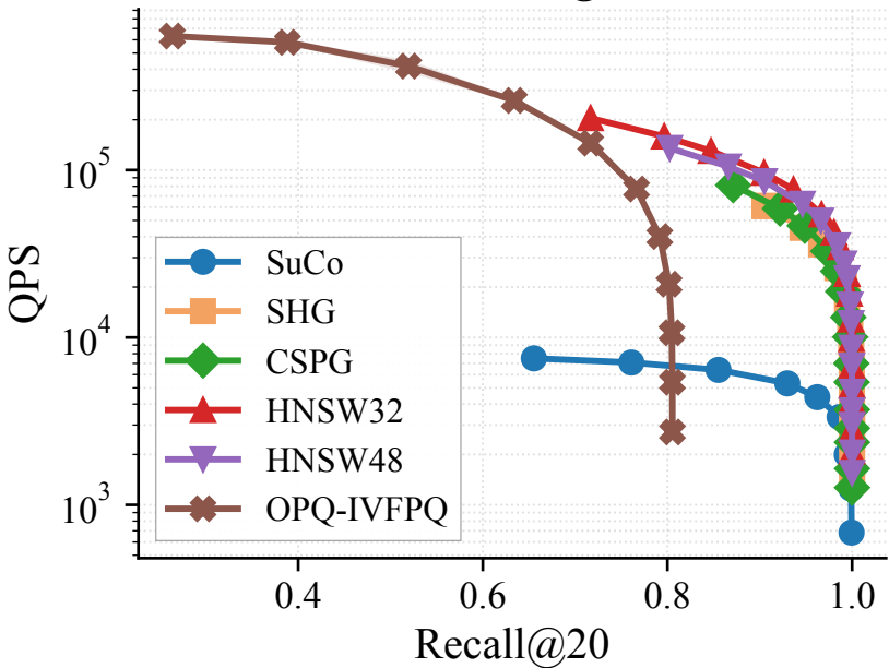
SIFT1M — Recall@20 vs QPS
