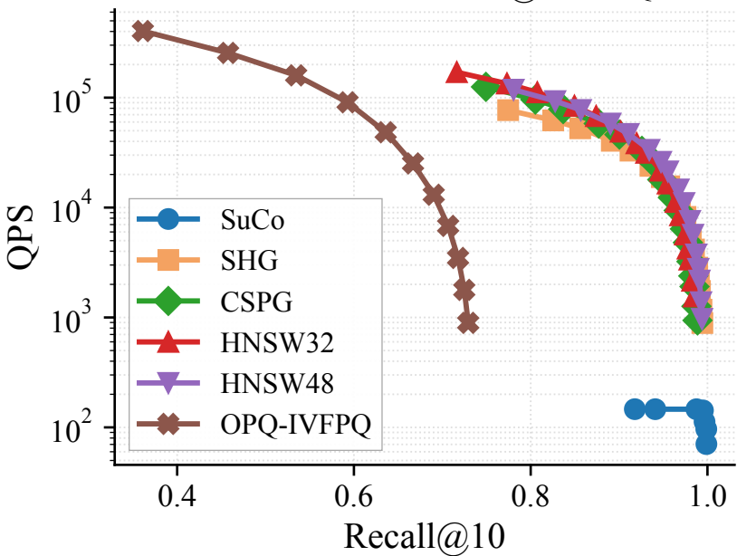
SPACEV10M — Recall@10 vs QPS
