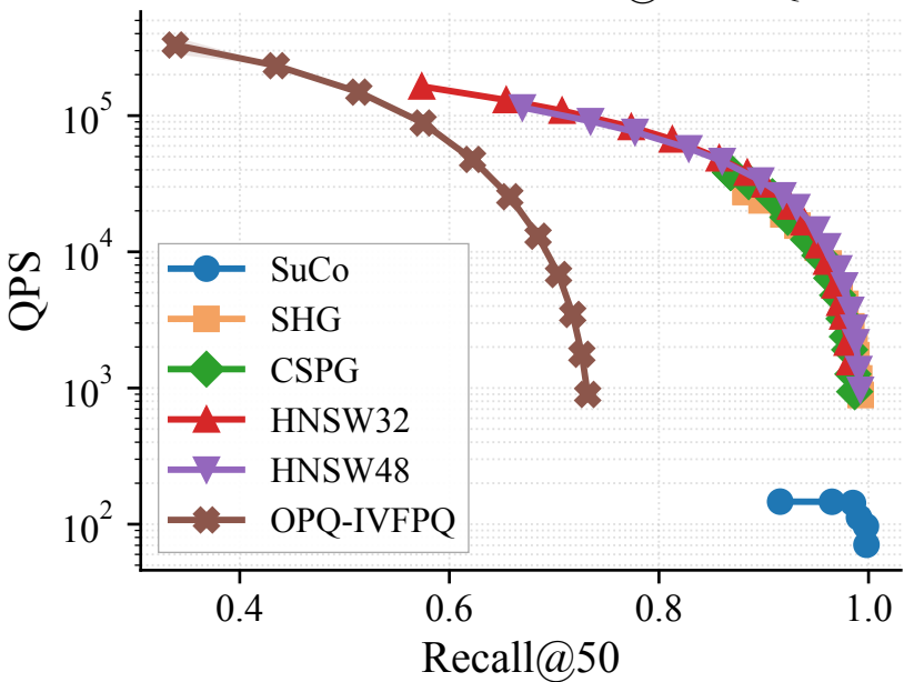
SPACEV10M — Recall@50 vs QPS
