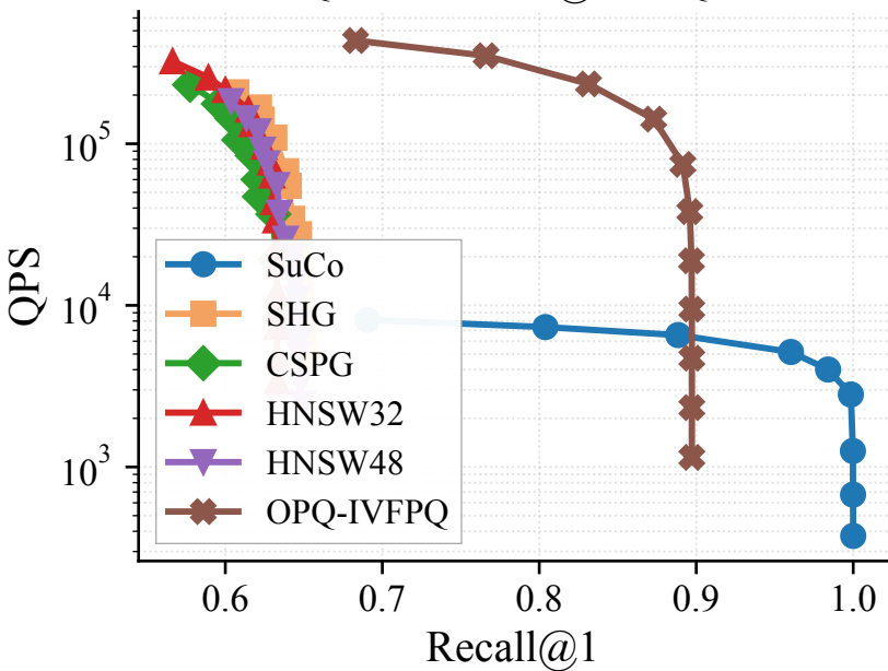
UQ-V — Recall@1 vs QPS
