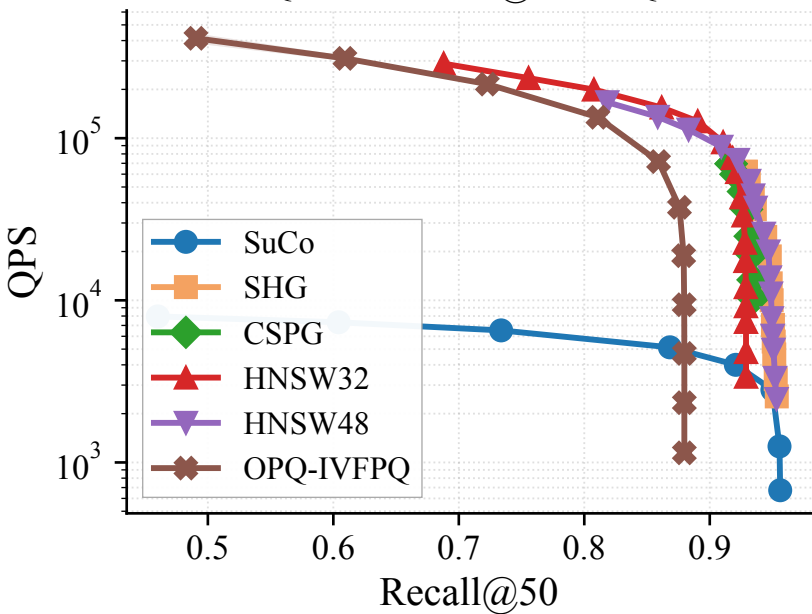
UQ-V — Recall@50 vs QPS
