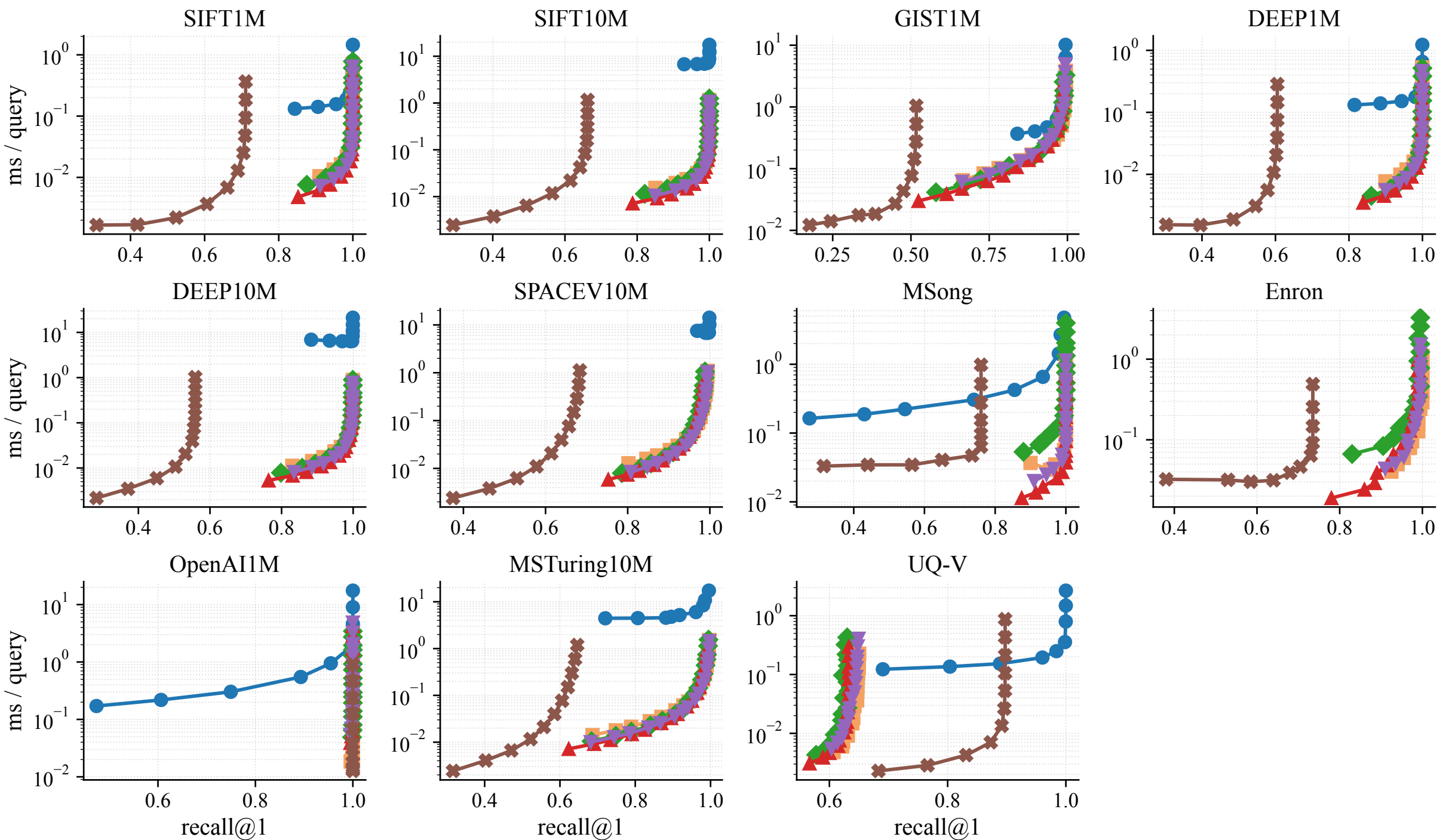
ms/query vs recall@1 (log-y)
