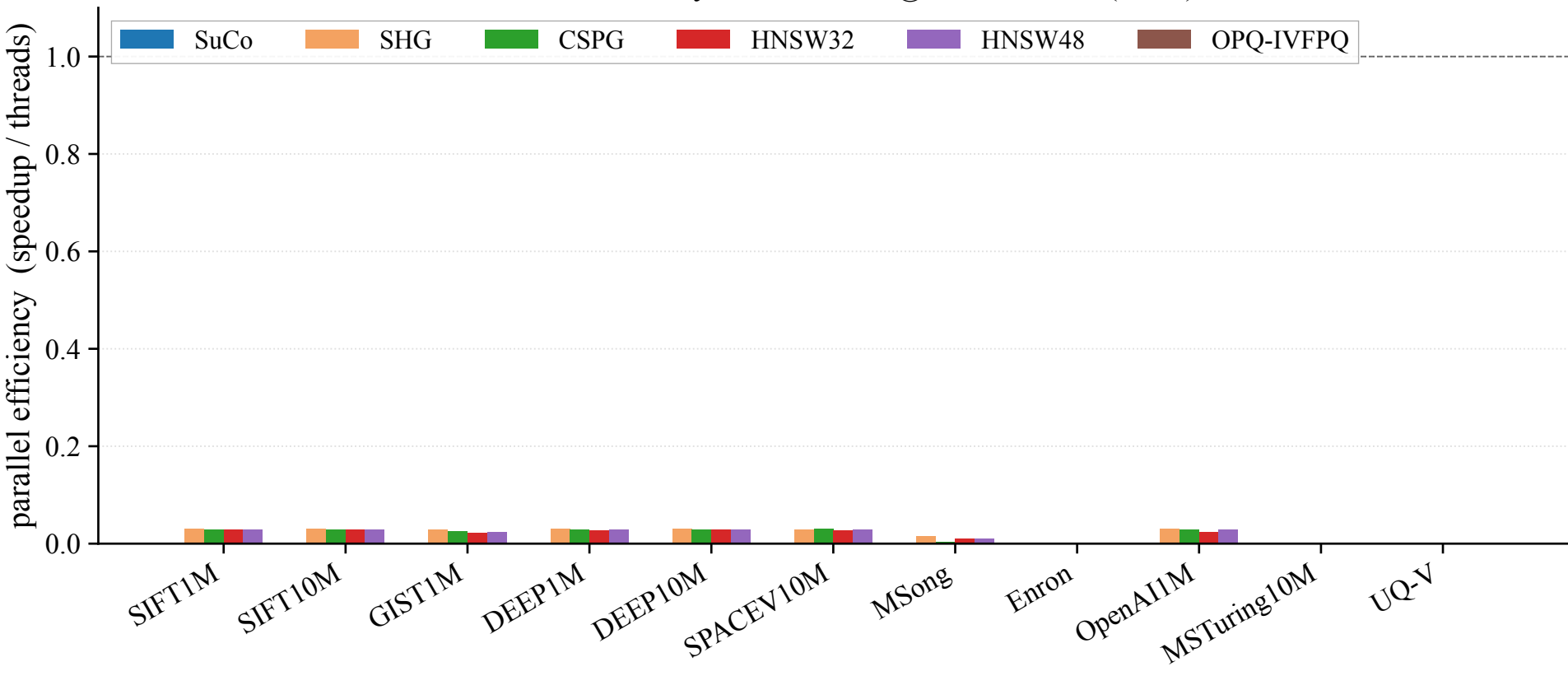
Parallel efficiency at 32 threads (@ recall \geq 0.95 (k=10))
