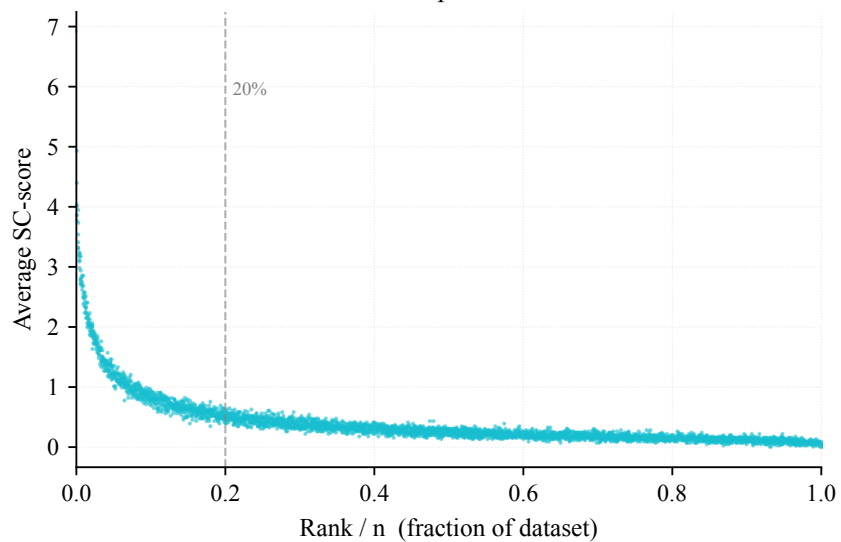
Deep10M
