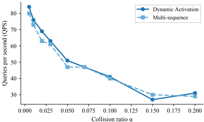
Dynamic Activation vs Multi-sequence (SIFT10M)
