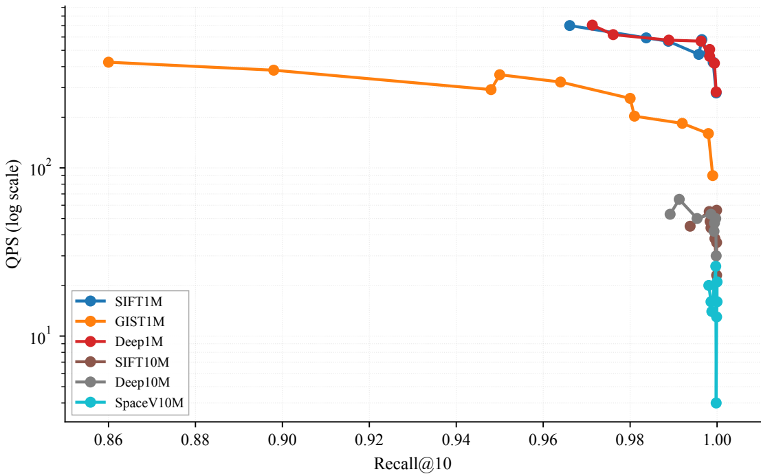
SuCo — Recall@10 vs QPS across all datasets
