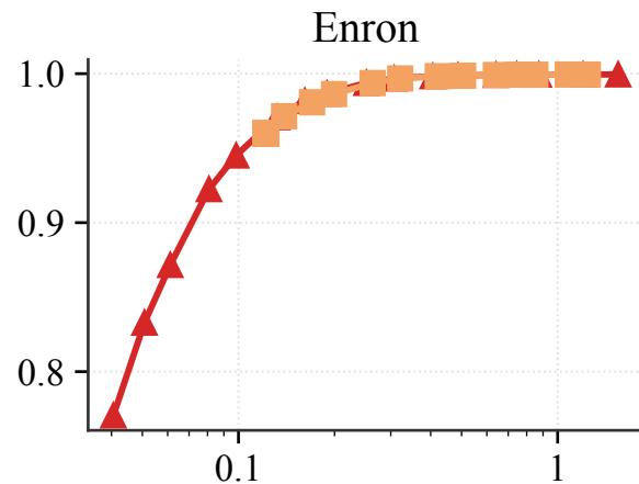
Recall@50 vs query time
