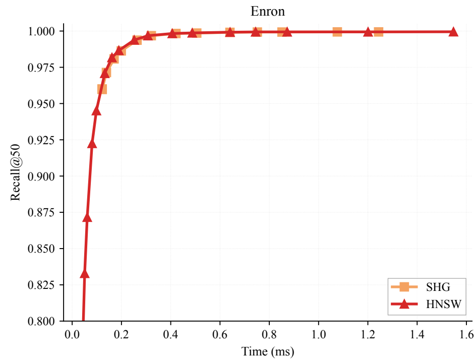
SHG vs HNSW — Recall vs Query Time (k=50)
