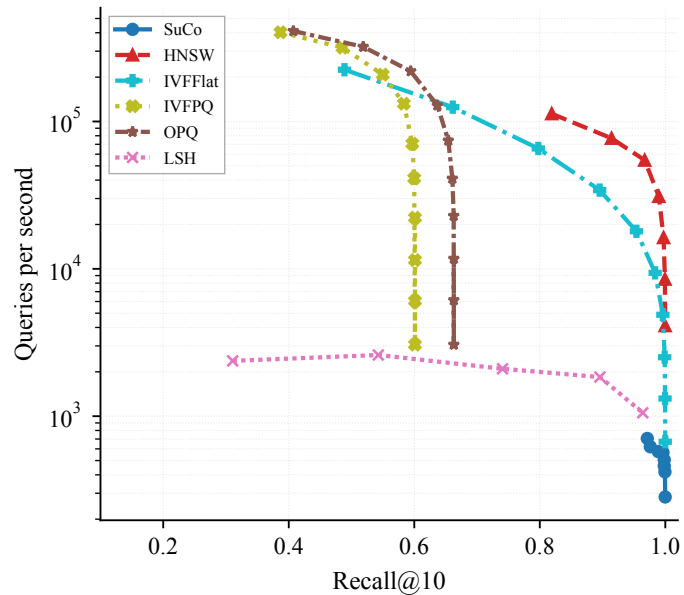
Deep1M (easy, d=96)
