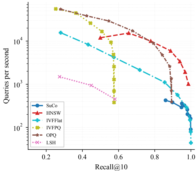
GIST1M (hard, d=960)
