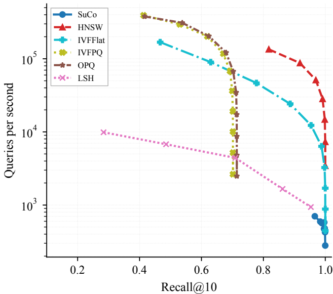
SIFT1M (easy, d=128)
