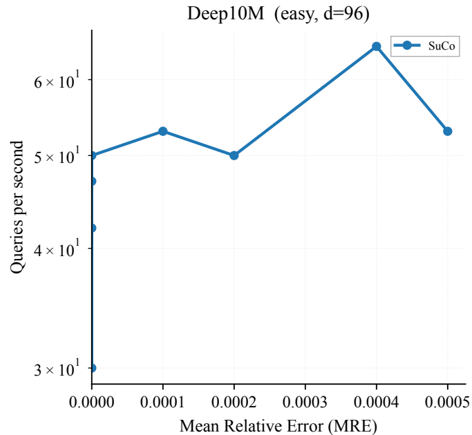
MRE vs QPS: 10M-scale datasets (SuCo)
