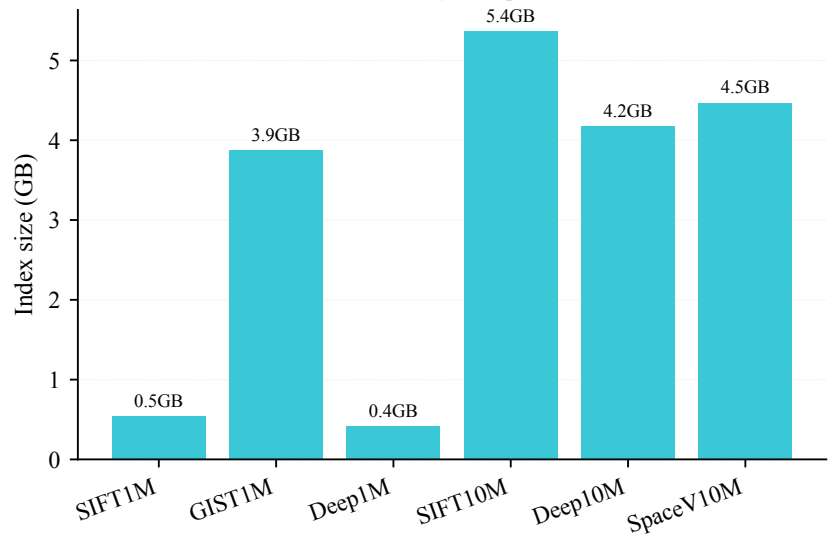
(b) Index memory footprint [SuCo]
