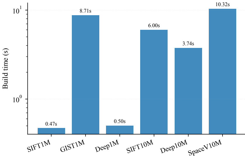
(a) Index build time [SuCo]
