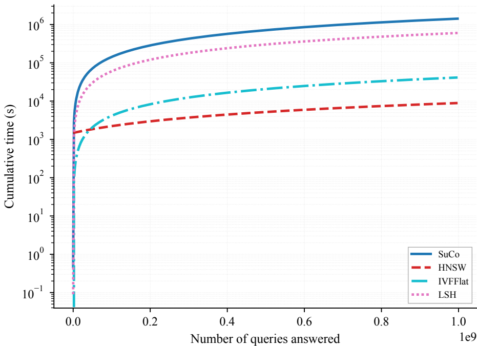
(c) SIFT10M, Recall \geq 0.8
