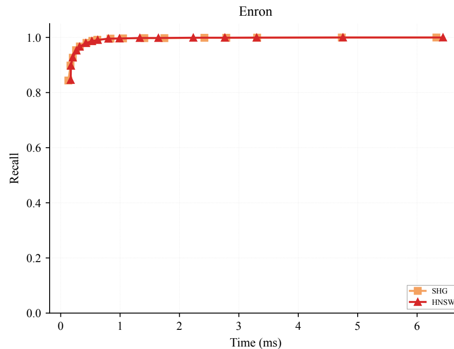
Ablation Study: Effect of Shortcuts and LB Pruning (k=20)
