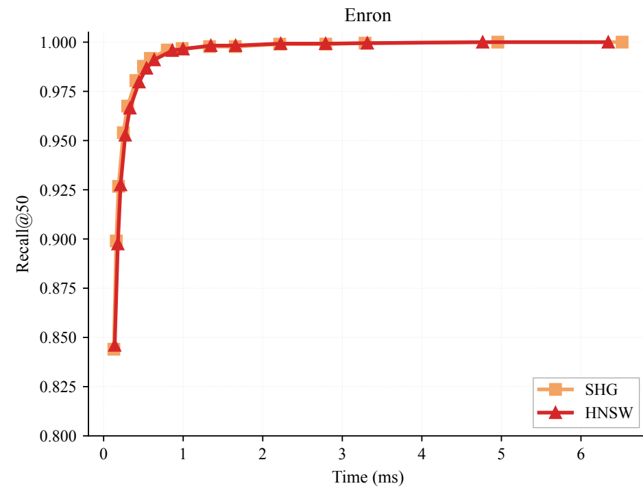
SHG vs HNSW — Recall vs Query Time (k=50)
