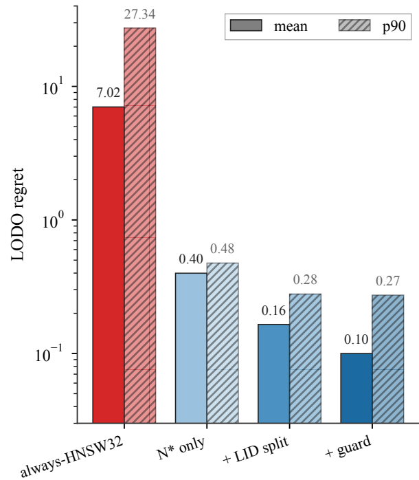
(c) stage ablation
