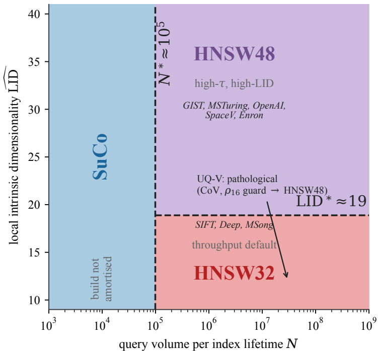
(a) fitted decision map ( \tau=0.99 )
