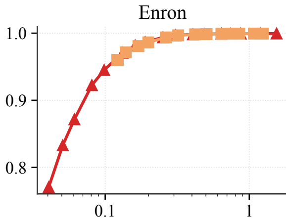
Recall@50 vs query time
