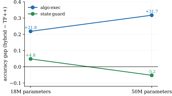
Figure 6: Accuracy gap at 18M vs. 50M (fixed training recipe, 2 seeds at 50M).
