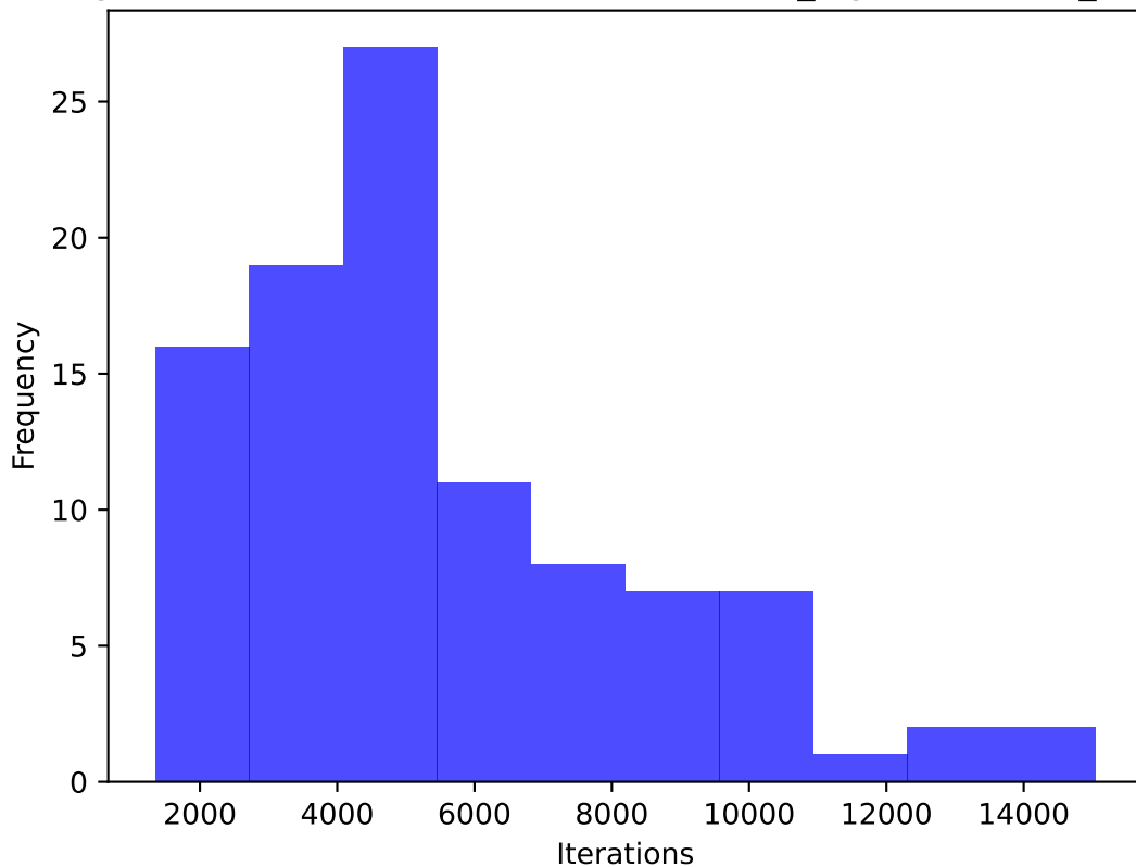
Histogram of Iterations to Reach Goal (search_algorithm=RRT_connect)
