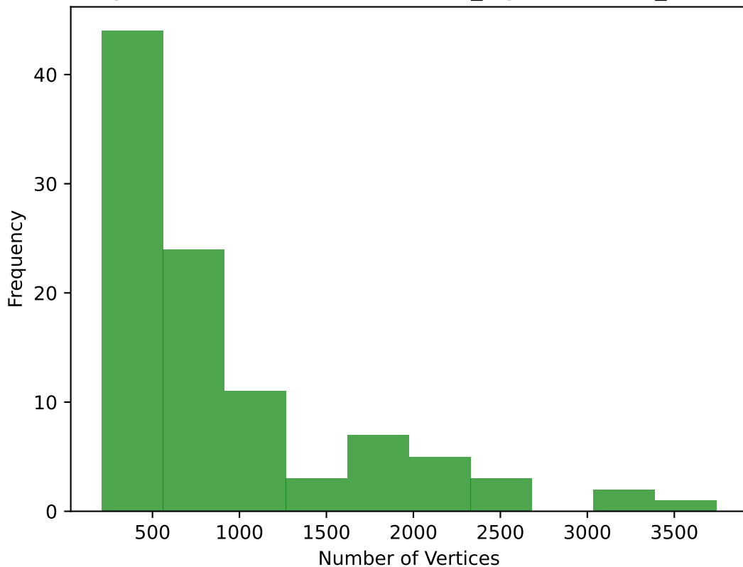
Histogram of Vertices in Tree (search_algorithm=RRT_connect)
