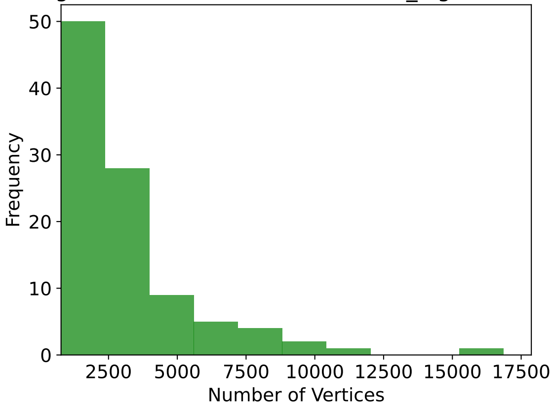
Histogram of Vertices in Tree (search_algorithm=RRT)
