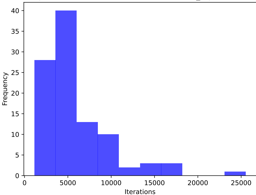
Histogram of Iterations to Reach Goal (search_algorithm=RRT)
