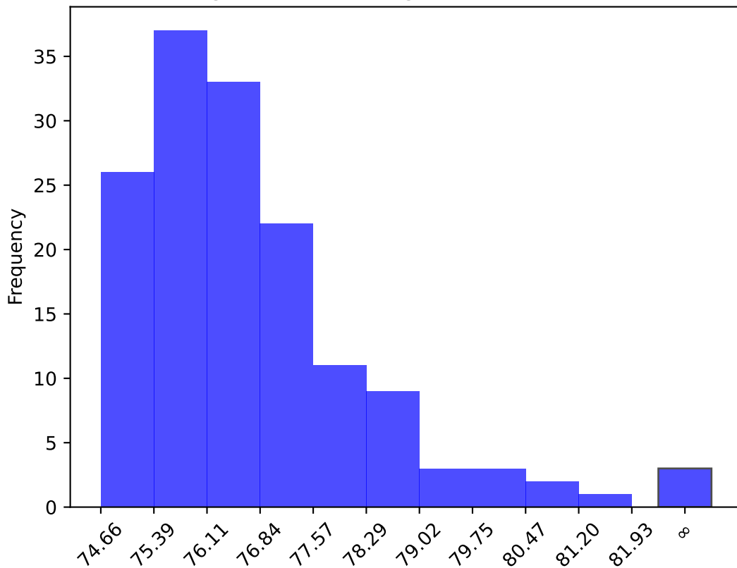
Histogram of Path Lengths at 1000 Iterations
