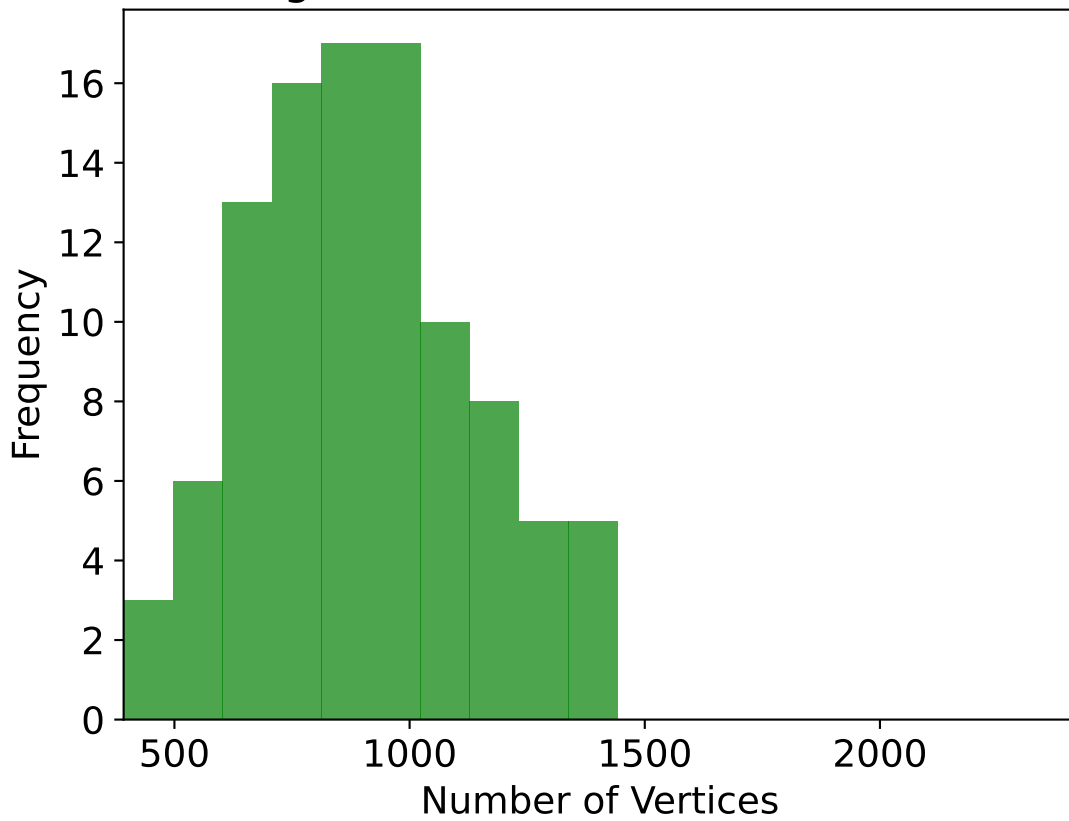
Histogram of Number of Vertices ( l=4 )
