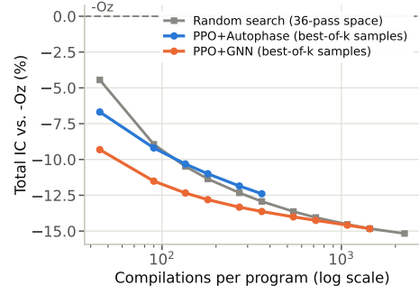
Fig. 1. Quality vs. budget across the 347 programs of the original battery (MiBench, CHStone, BLAS, csmith, NPB, POJ-104), summed IC relative to -\text{Oz} : best-of- k sampling (GNN k=1..32 , Autophase k=1..8 , mean over three seeds) vs. expected best-of- k random search.
