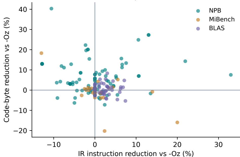
Same IC-selected portfolio candidate
