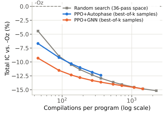
Fig. 1. Quality vs. budget across all 347 battery programs (MiBench, CHStone, BLAS, csmith, NPB, POJ-104), summed IC relative to -Oz : best-of- k sampling (GNN k=1..32 , Autophase k=1..8 , mean over three seeds) vs. expected best-of- k random search.
