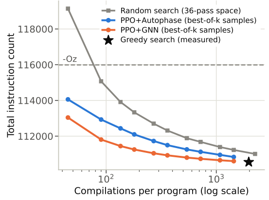
Fig. 1. Quality vs. budget on cBench val+test: best-of- k sampling ( k=1..32 ) vs. expected best-of- k random search and measured greedy search.
