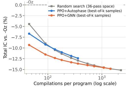
Fig. 1. Quality vs. budget across all 347 battery programs (MiBench, CHStone, BLAS, csmith, NPB, POJ-104), summed IC relative to -Oz : best-of- k sampling (GNN k=1\text{--}32 , Autophase k=1\text{--}8 , mean over three seeds) vs. expected best-of- k random search.
