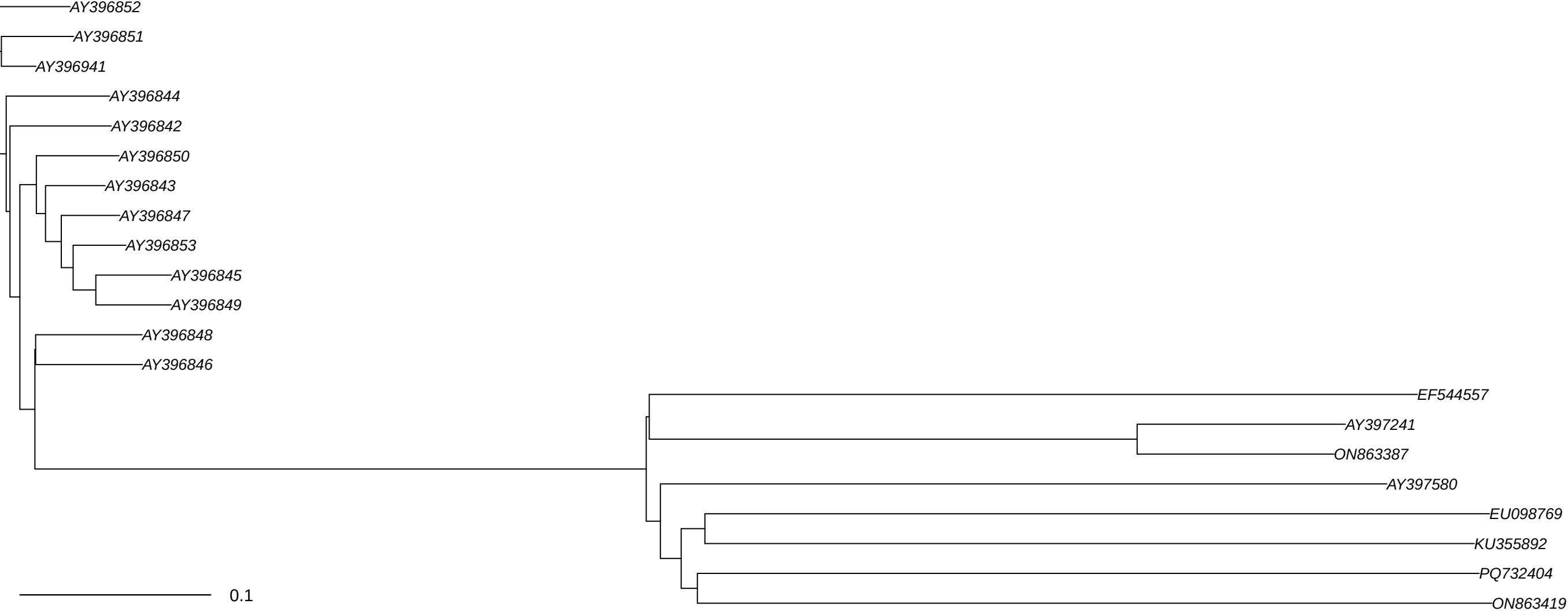
Neighbor-Joining tree: gh80_matrix
