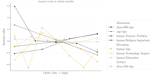
Figure 6: Polarization attribution trends in ordinal groups. The left side of the x-axis (low orders) refers to young annotators, low education, low religiousness, and indifference towards the impacts of toxicity and technology. The full ordinal modes for each dimension and their individual labels can be found in App. F.
