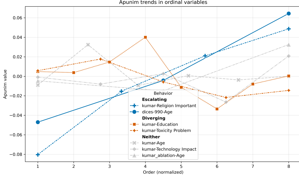
Fig. 8: The behavior of ordinal variables in all datasets. The x-axis represents the order of each factor (marked as 1), 2), . . . in Tables 7a,7b,1,7c). The x-axis is normalized to the smallest common denominator between the number of ordinal values.
