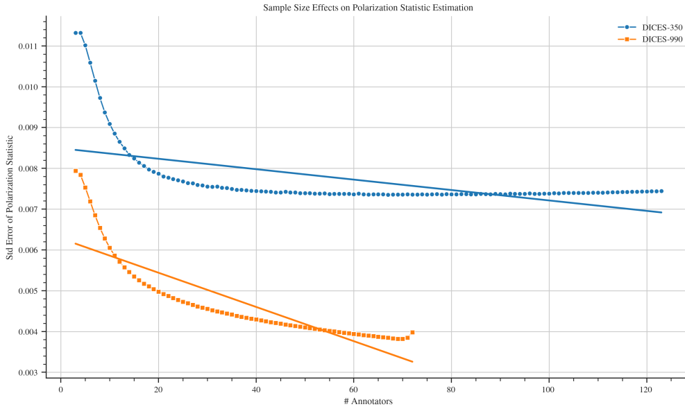
Fig. 9: Standard error of the pol-statistic when sampled with replacement for various number of annotators.
