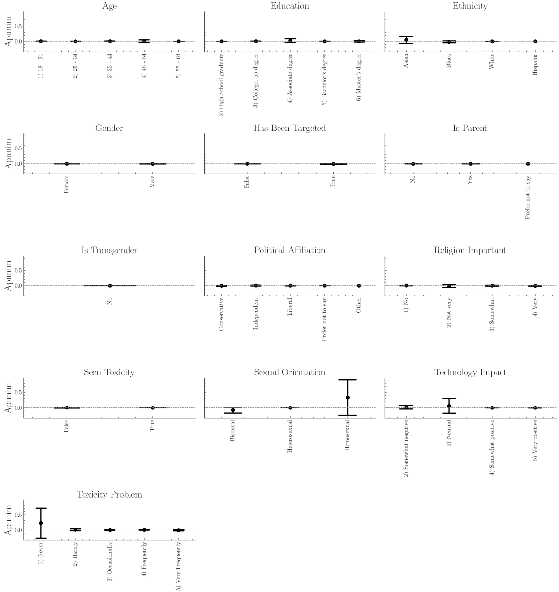
Fig. 9. Apunim values on the Kumar dataset ( n_{\text{samples}} = 1000 ) across ten runs with different subsets. Black bars indicate two SDs. PC dimensions with many groups are more volatile, although all dimensions broadly keep the same apunim sign across subsets.
