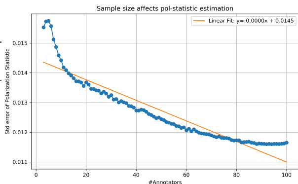
Figure 6: Standard error of the pol\text{-}statistic when sampled with replacement from the 100-annotator synthetic dataset for various numbers of annotators. We use the 100-annotator synthetic dataset and sample progressively 3 – 100 annotators with replacement, then calculate the standard error with the mean pol\text{-}statistic . As expected, the standard error is inversely proportional to the number of annotators, although the difference is not great, even for a low number of annotators.
