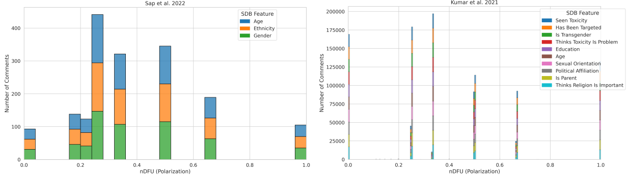
Figure 5: Histogram of dataset polarization for the human datasets considered in this paper per SDB feature.
