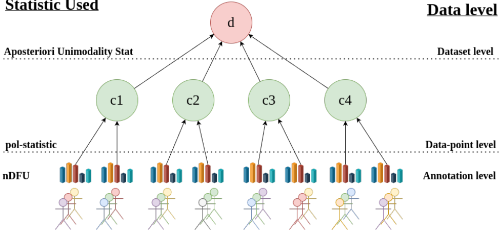
Fig. 5: An overview of how annotation information is sequentially aggregated for the Apunim metric. We gather statistical information from the annotations (different PCs are denoted by different colors) via the nDFU measure, which is aggregated by the pol apriori and pol observed statistics for each datapoint. We aggregate these statistics on the dataset level, and compare them to get a chance-corrected Apunim value.
