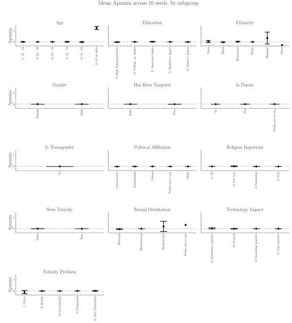
Figure 9: Apunim values on the Kumar dataset ( n_{samples} = 3000 ) across ten runs with different subsets. Black bars indicate two SDs. PC dimensions with many groups are more volatile, although all dimensions broadly keep the same apunim sign across subsets.
