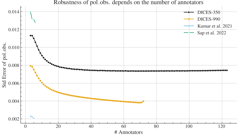
Fig. 8 Std error of the pol_{obs} statistic (Equation 2) when sampled with replacement for various number of annotators. We repeat the sampling process thirty times, and plot the average pol_{obs} value.
