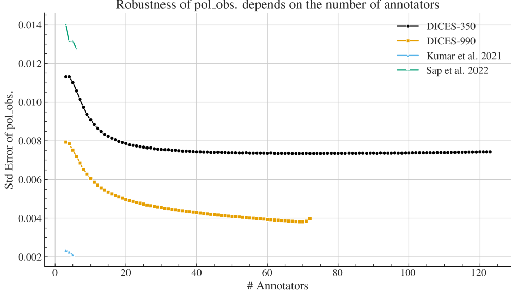
Fig. 7 Standard error of the mean pol_{obs} (Eq. 3) across increasing sample sizes. The x-axis shows the sample size (number of annotators), starting from 3 and increasing one at a time, up to the largest annotator count for which a sufficient number of items exists. For each sample size, we draw 30 samples (with replacement) and compute the mean of pol_{obs} ; the plotted values represent the resulting standard error of that mean.
