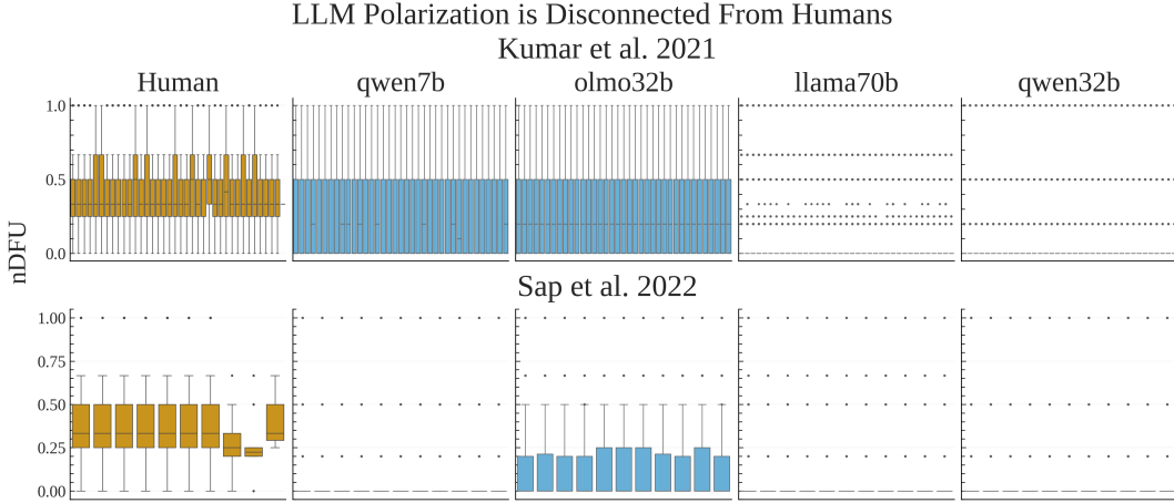
Figure 6: nDFU grouped by dataset (rows) and model family (columns) for each PC persona dimension in the primary annotation task (blue) using the default prompt, compared with human annotations on the same sample (yellow).
