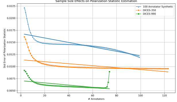
Figure 8: Standard error of the pol-statistic when sampled with replacement from the 100 LLM-annotator synthetic dataset for various number of annotators.
