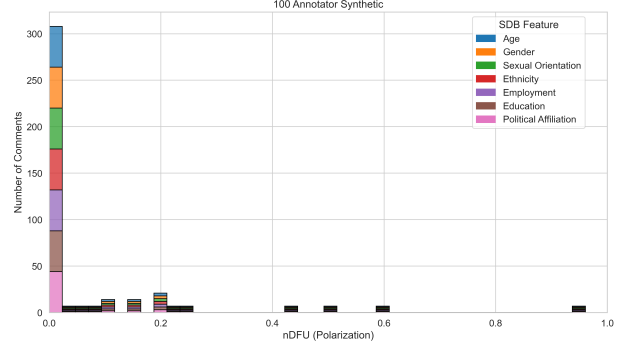
Figure 9: Histogram of dataset polarization for the Sap et al. [17] annotated by 100 LLM annotators dataset considered in this paper per SDB feature.
