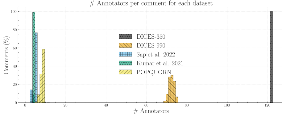
Fig. 6. We calculate the ratio of items for each dataset (y-axis) that had x number of annotators (x-axis). We truncate the x-axis to 130 annotators, disregarding very few items in the Kumar dataset exceeding this threshold (see Table 6), which is likely caused by a data error.
