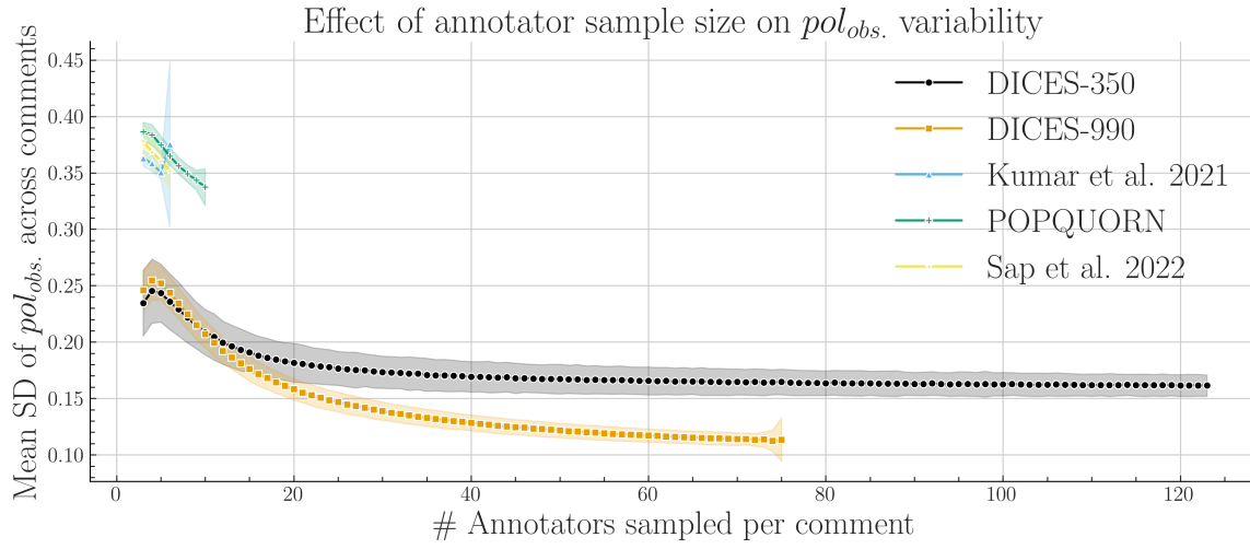
Fig. 11. SD of pol_{obs} across items, averaged across 1000 runs. Shaded areas represent two SDs. Pol. estimates benefit from more annotators up to n = 20 , at which point they begin to plateau.
