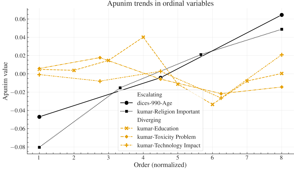
Fig. 6 Apunim value per ordinal variable across datasets with more than one statistically significant value. The x-axis represents the order of each factor, marked by the respective number in Tables 2-5. The x-axis is normalized to the smallest common denominator between the number of ordinal values.
