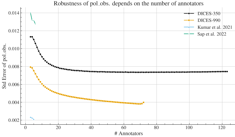
Fig. 7 The standard error of the mean when sampling (with replacement) for various annotator numbers, repeating sampling thirty times, when measuring the (average of) pol_{obs} (Eq. 3).
