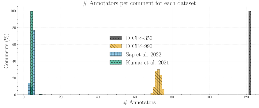
Figure 8: We calculate the ratio of items for each dataset (y-axis) that had x number of annotators (x-axis). We truncate the x-axis to 130 annotators, disregarding very few items in the Kumar dataset exceeding this threshold (see Table 3), which is likely caused by a data error.
