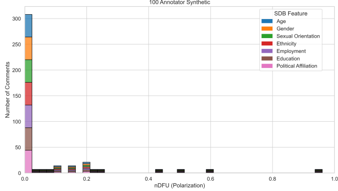
Fig. 8 Histogram of dataset polarization for the [4] annotated by 100 LLM annotators dataset considered in this paper per SDB feature.
