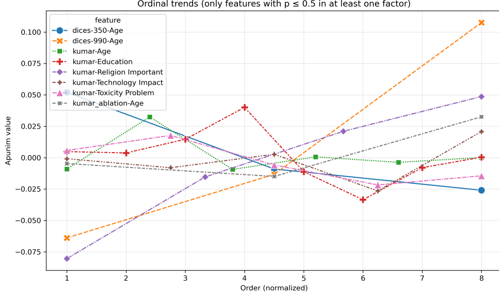
Fig. 7 The behavior of ordinal variables in all datasets. The x-axis represents the order of each factor (marked as 1), 2), ... in Tables 2,3,5,4). The x-axis is normalized to the smallest common denominator between the number of ordinal values.
