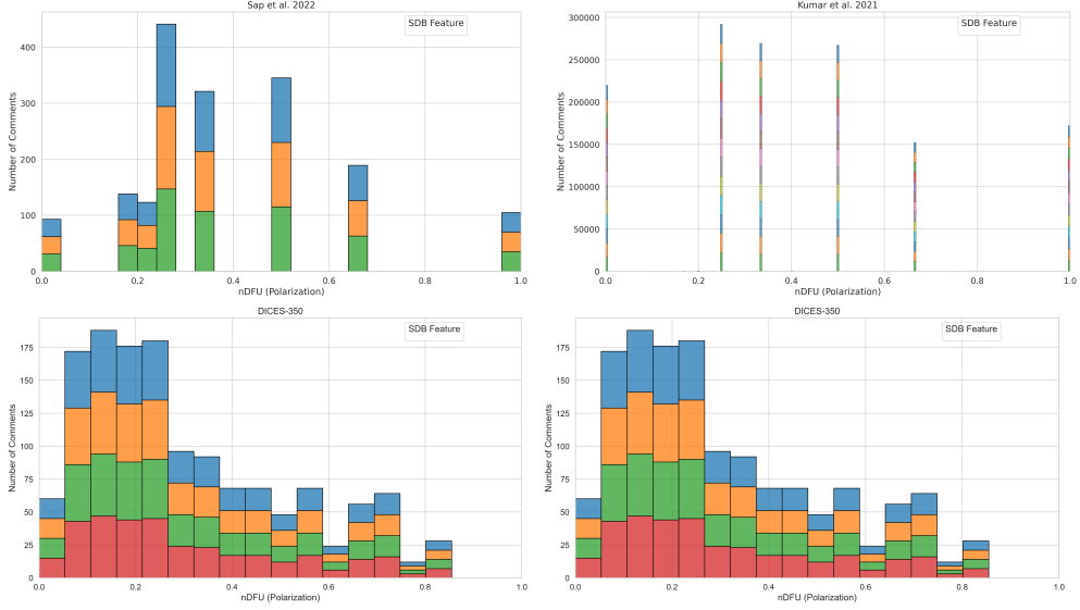
Fig. 6 Histogram of dataset polarization for the human datasets considered in this paper per SDB feature.
